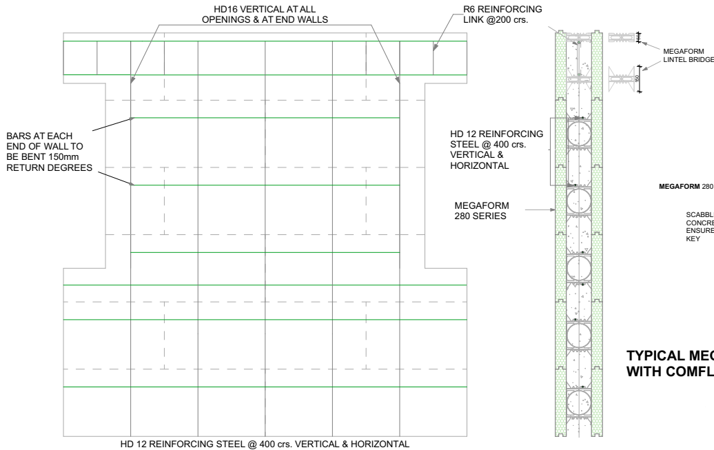
WALL ELEVATION
