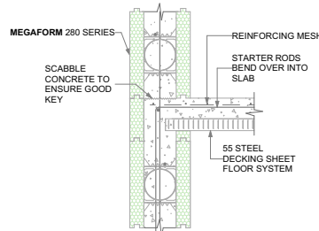
TYPICAL MEGAFORM WALL CONSTRUCTION WITH COMFLOR STEEL DECKING SYSTEM
