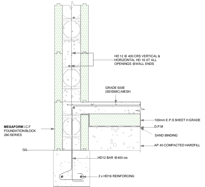
TYPICAL MEGAFORM FOUNDATION DETAIL WITH MEGAFORM I.C.F WALL
