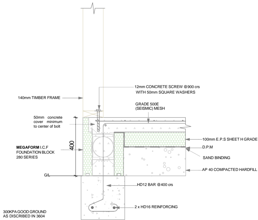
TYPICAL MEGAFORM FOUNDATION DETAIL WITH 140mm TIMBER FRAME
