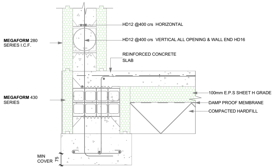
MEGAFORM FOUNDATION 430 SERIES WITH MEGAFORM I.C.F 280 SERIES WALL
