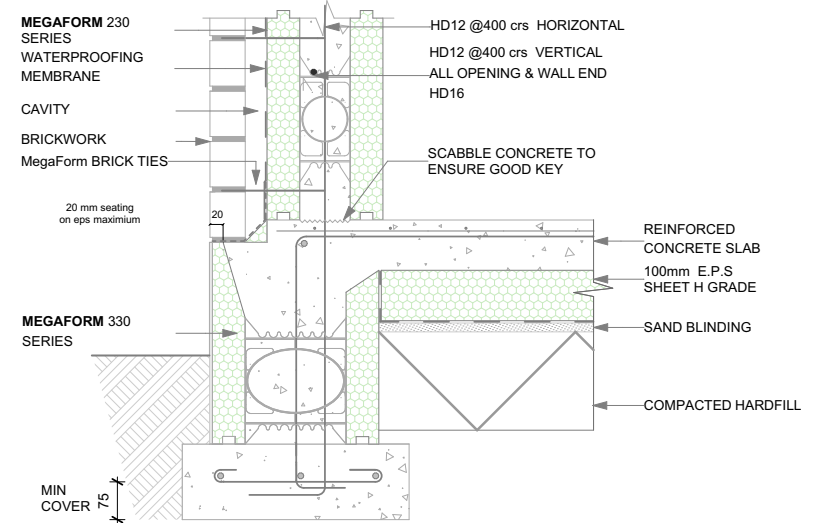
MEGAFORM FOUNDATION 330 SERIES AND MEGAFORM I.C.F 230 SERIES WALL WITH BRICKWORK CLADDING
