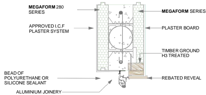
WINDOW HEAD
