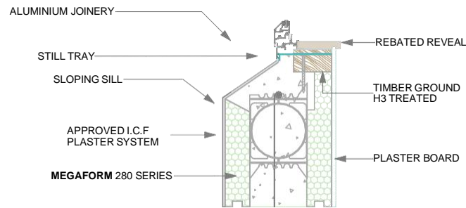
WINDOW SILL
