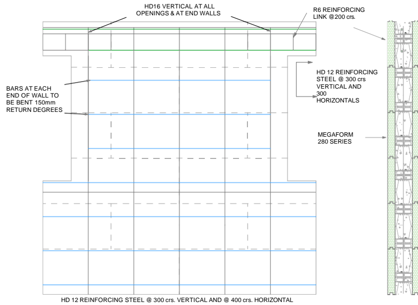
WALL ELEVATION
