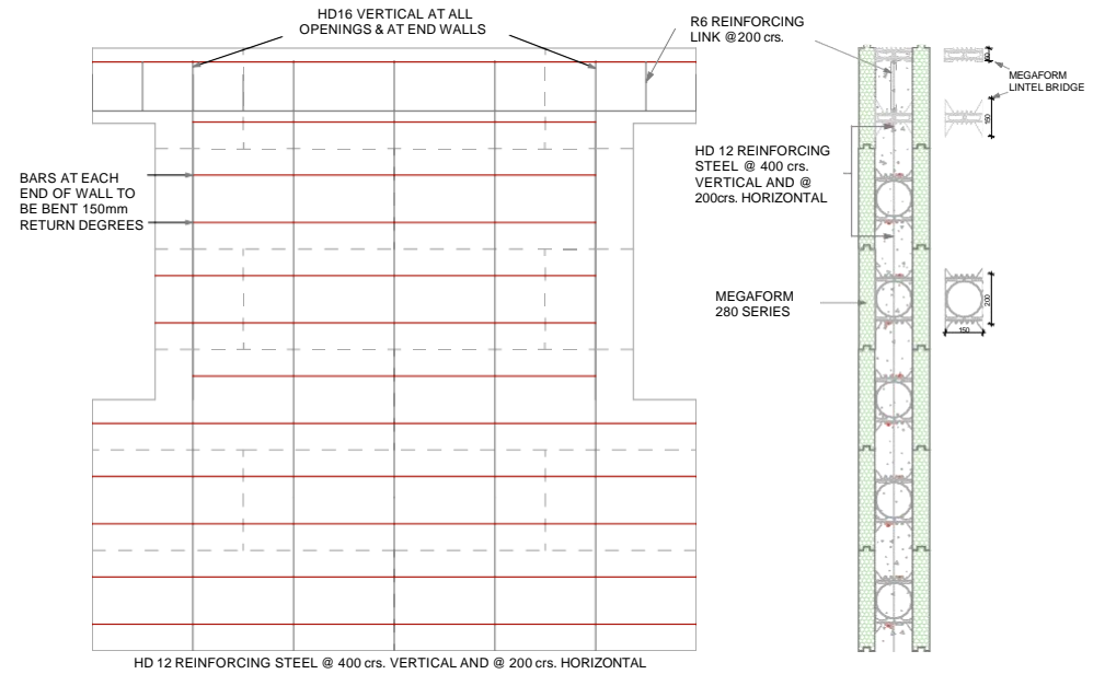
WALL ELEVATION
