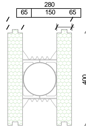
MEGAFORM SERIES 280
