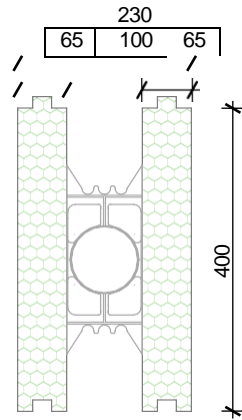
MEGAFORM SERIES 230
