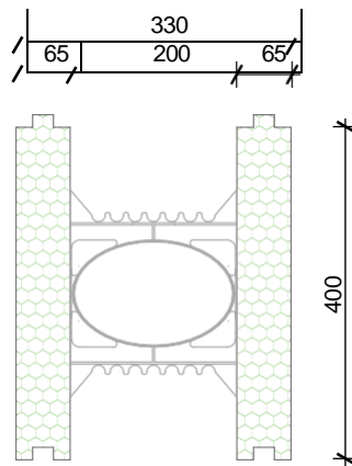
MEGAFORM SERIES 330
