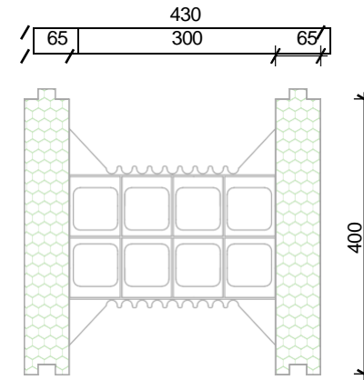
MEGAFORM SERIES 430
