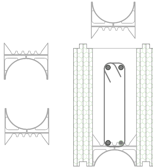
HALF BRIDGE FOR LINTEL STEEL PLACEMENT
