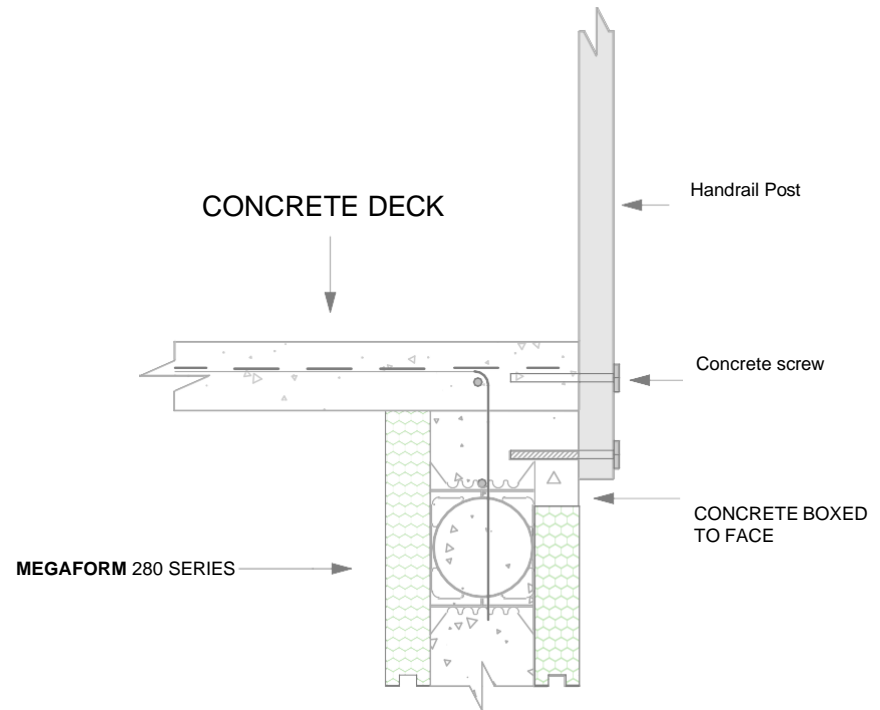
FACED FIXED HANDRAIL POST
