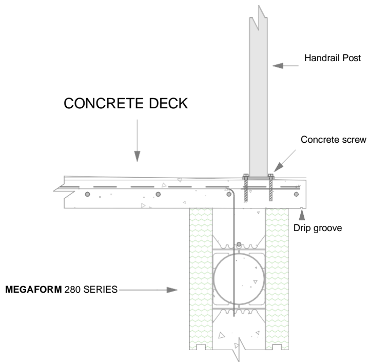
TOP FIXED HANDRAIL POST
