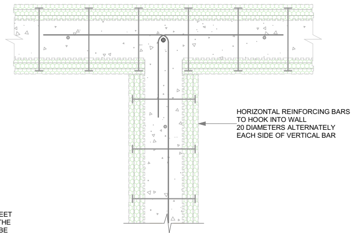
MEGAFORM WALLS JUCTION
