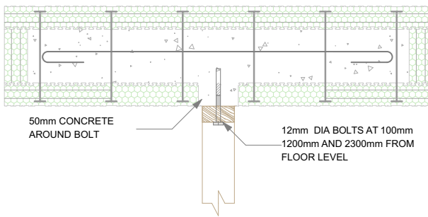
TIMBER WALL / MEGAFORM WALL JUNCTION
