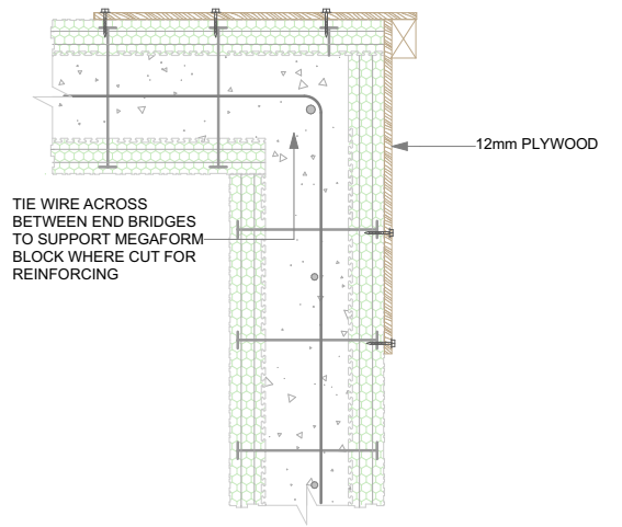
CORNERS WITHOUT CORNER BLOCKS
