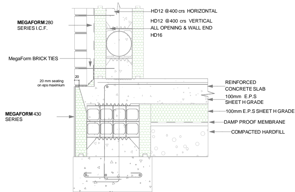
MEGAFORM FOUNDATION 430 SERIES AND MEGAFORM 280 SERIES WALL WITH BRICK CLADDING
