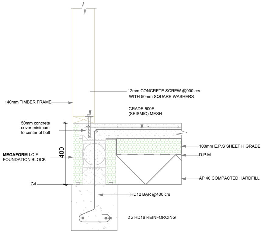
TYPICAL MEGAFORM FOUNDATION DETAIL WITH 140mm TIMBER FRAME
