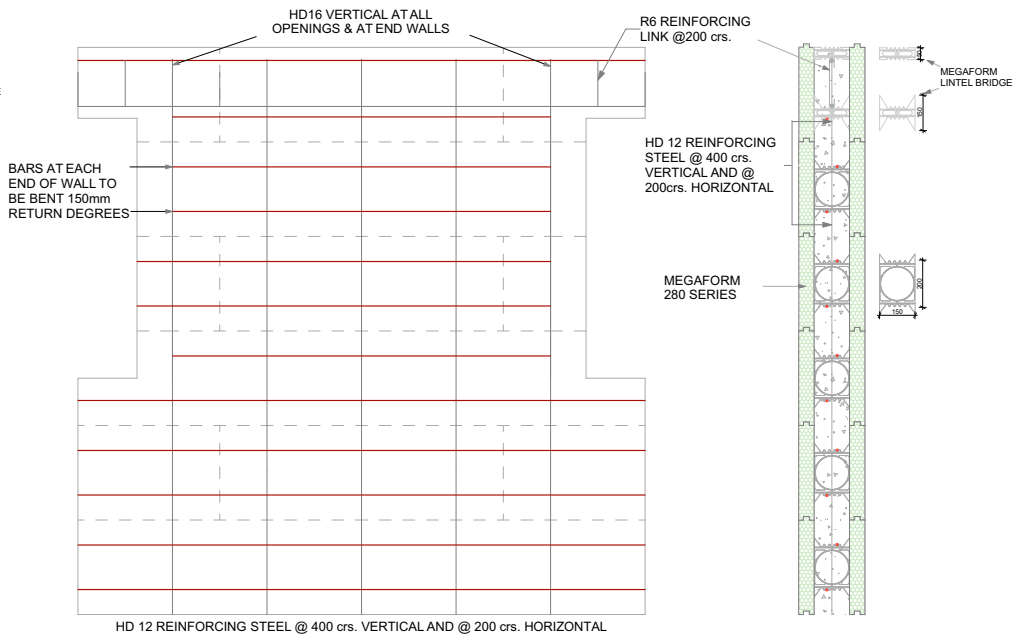
WALL ELEVATION
