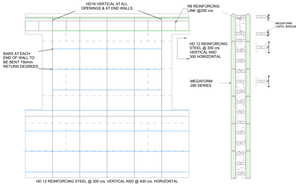
WALL ELEVATION
